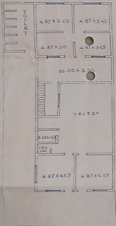
G.F. PLAN
